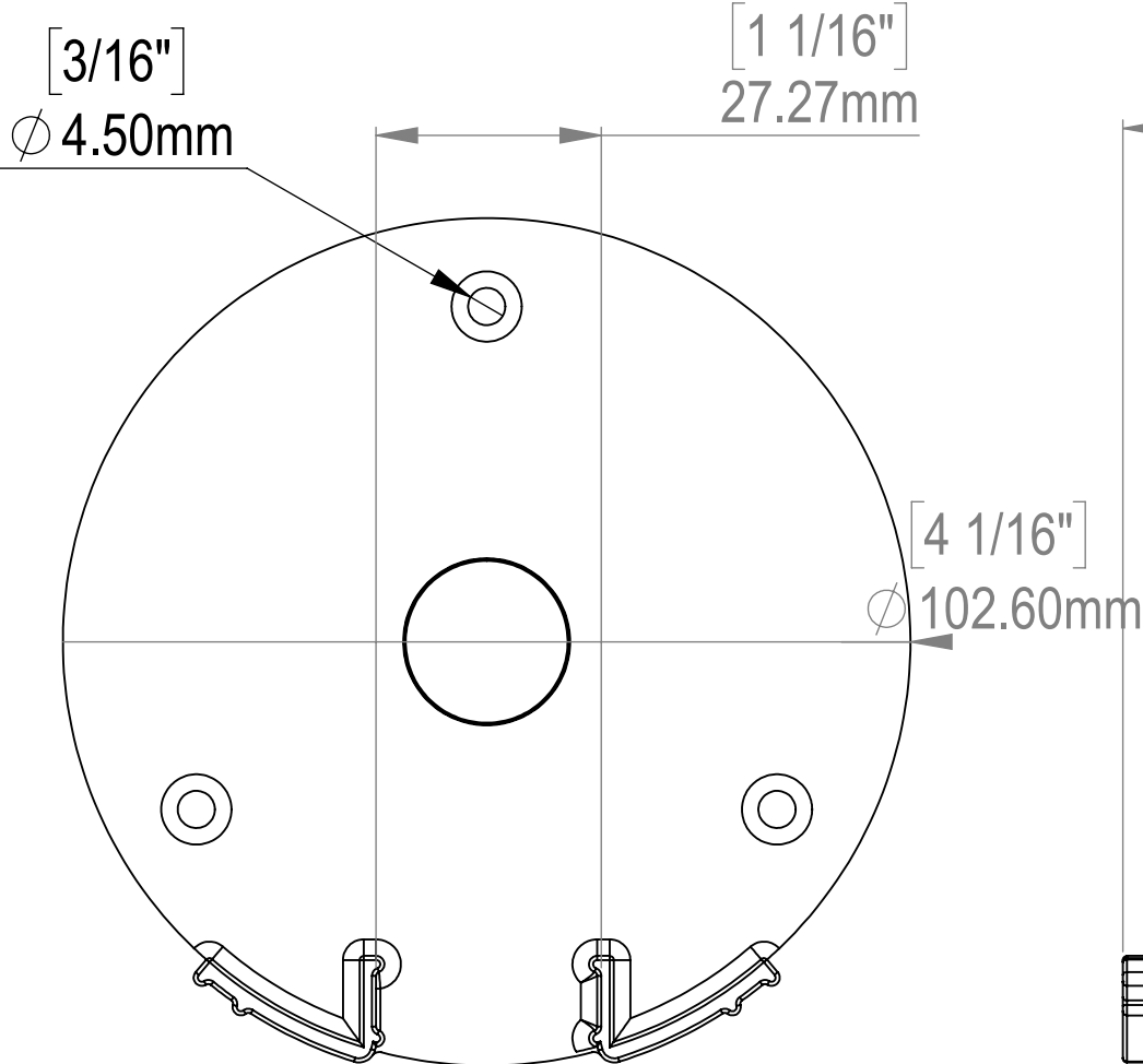
Front View
